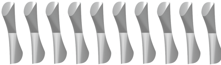
Fig. 3 Zariski closure X_j of S_{\ell_j} (Example 3.2)
